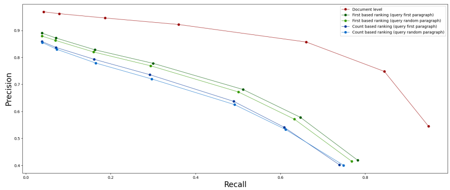
Fig. 3: Different configurations for the TF-IDF-based approach on the test set
